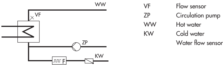
Fig. 11 · Schematics of an instantaneous heating system with water flow sensor (CO4 -> F04 - 1, select: AnA)
